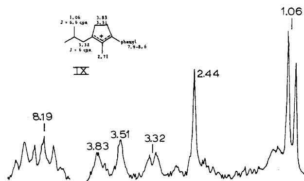
Fig. 4.—N.m.r. spectrum of IX in 96% H 2 SO 4 .
