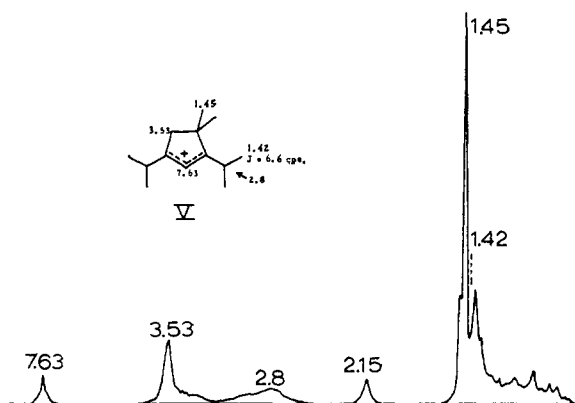
Fig. 2.—N.m.r. spectrum of V in 96% H 2 SO 4 formed by adding 2,3,3-trimethylborneol (IV) to 96% H 2 SO 4 .
