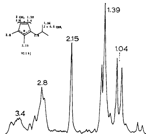
Fig. 3.—N.m.r. spectrum of VI in 96% H 2 SO 4 .
