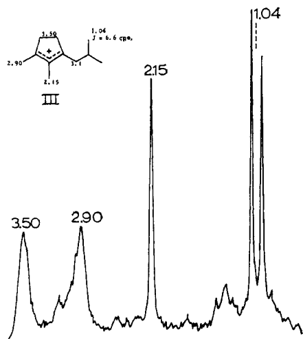
Fig. 1.—N.m.r. spectrum of III in 96% H 2 SO 4 formed by adding 2-methylfenchol or 2-methylborneol to 96% H 2 SO 4 .
